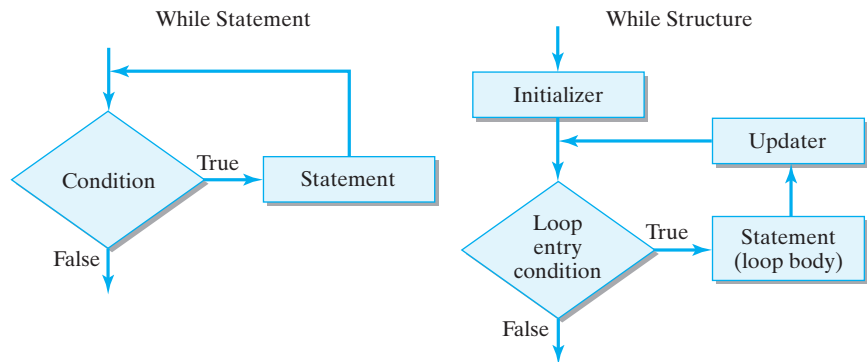
Figure 3.15: Flowchart of the while statement and while structure.
