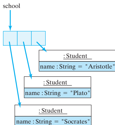
Figure 9.3: An array of Students .
