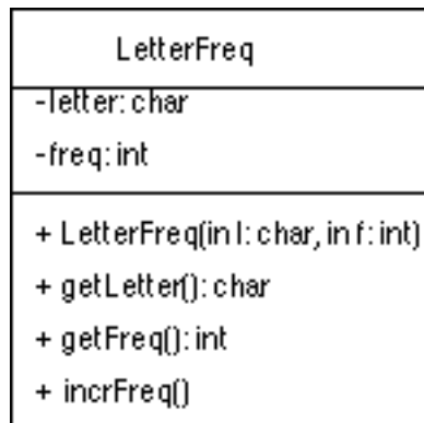
Figure 9.9: UML for LetterFreq .
