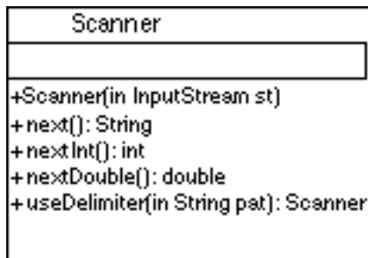
Figure 2.25: The Scanner class, with a partial list of its public methods.
