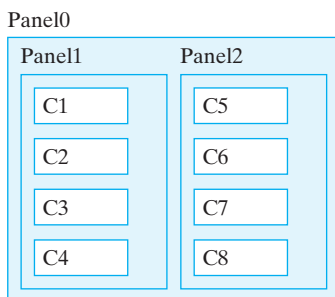
Figure 13.28: Complex layouts can be achieved by nesting containers that use the BoxLayout .
