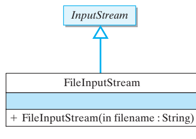
Figure 11.20: The java.io.FileInputStream class.
