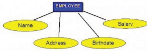
Figure 8.2. How attributes are represented in an ERD.
