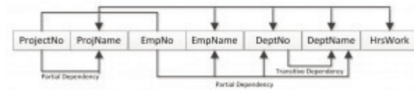
Figure 11.6. Dependency diagram.
