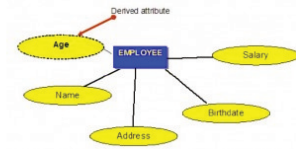
Figure 8.5. Example of a derived attribute.
