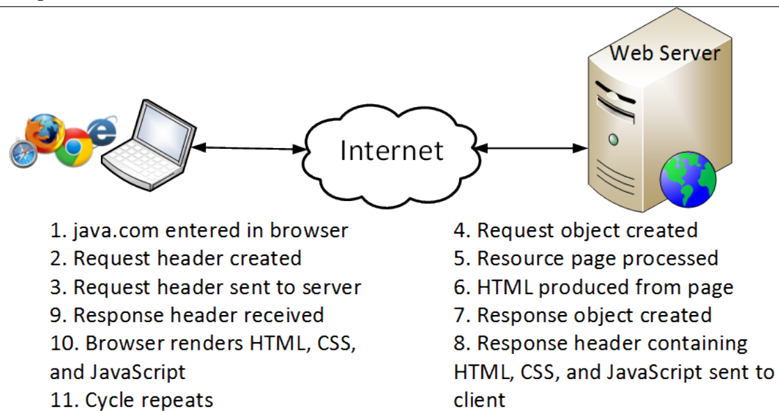
Image 3 . Browser and Server Communication
