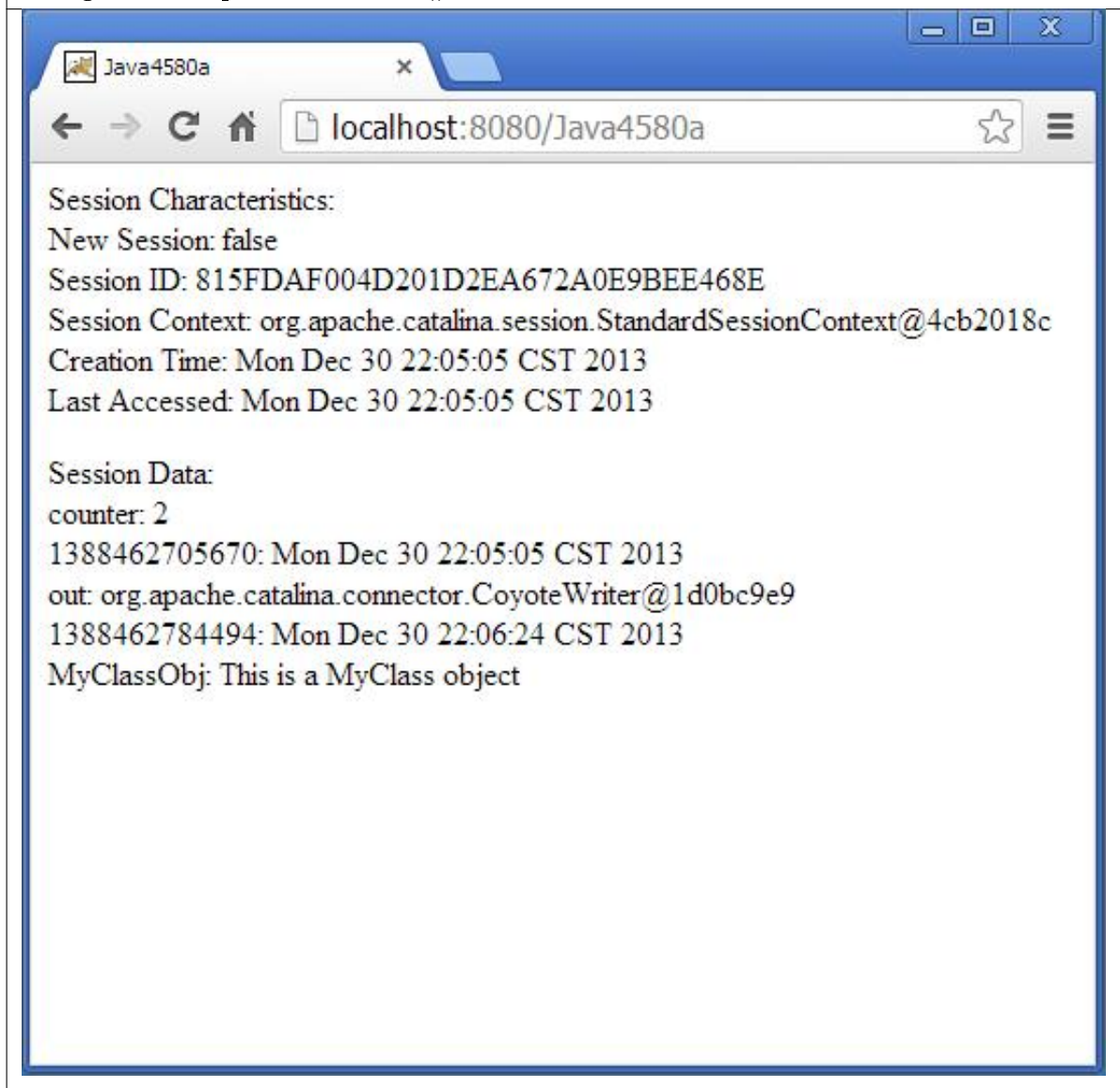
Image 2 . Output from access #2.
