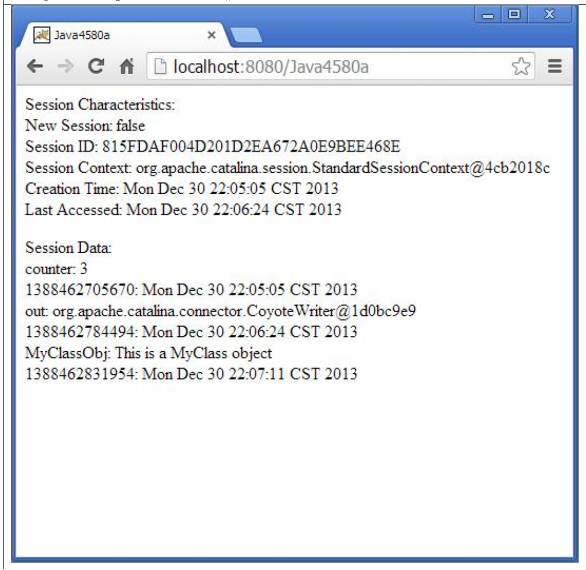
Image 3 . Output from access #3.
